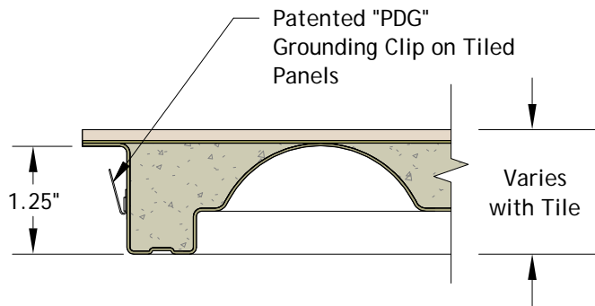
TILE COVERED PANEL
