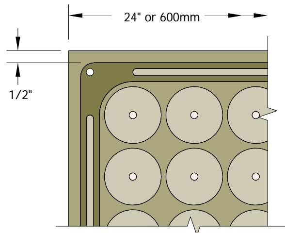
PARTIAL BOTTOM VIEW
