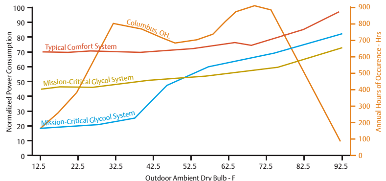
Full System Power Comparison - 100% Load
