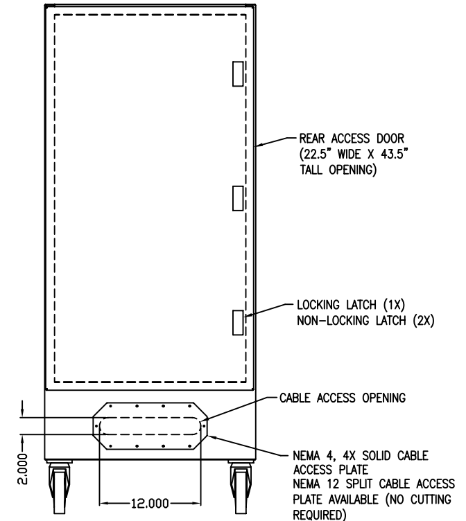
REAR VIEW
