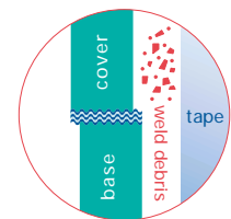
Conventional Ultrasonic Weld
